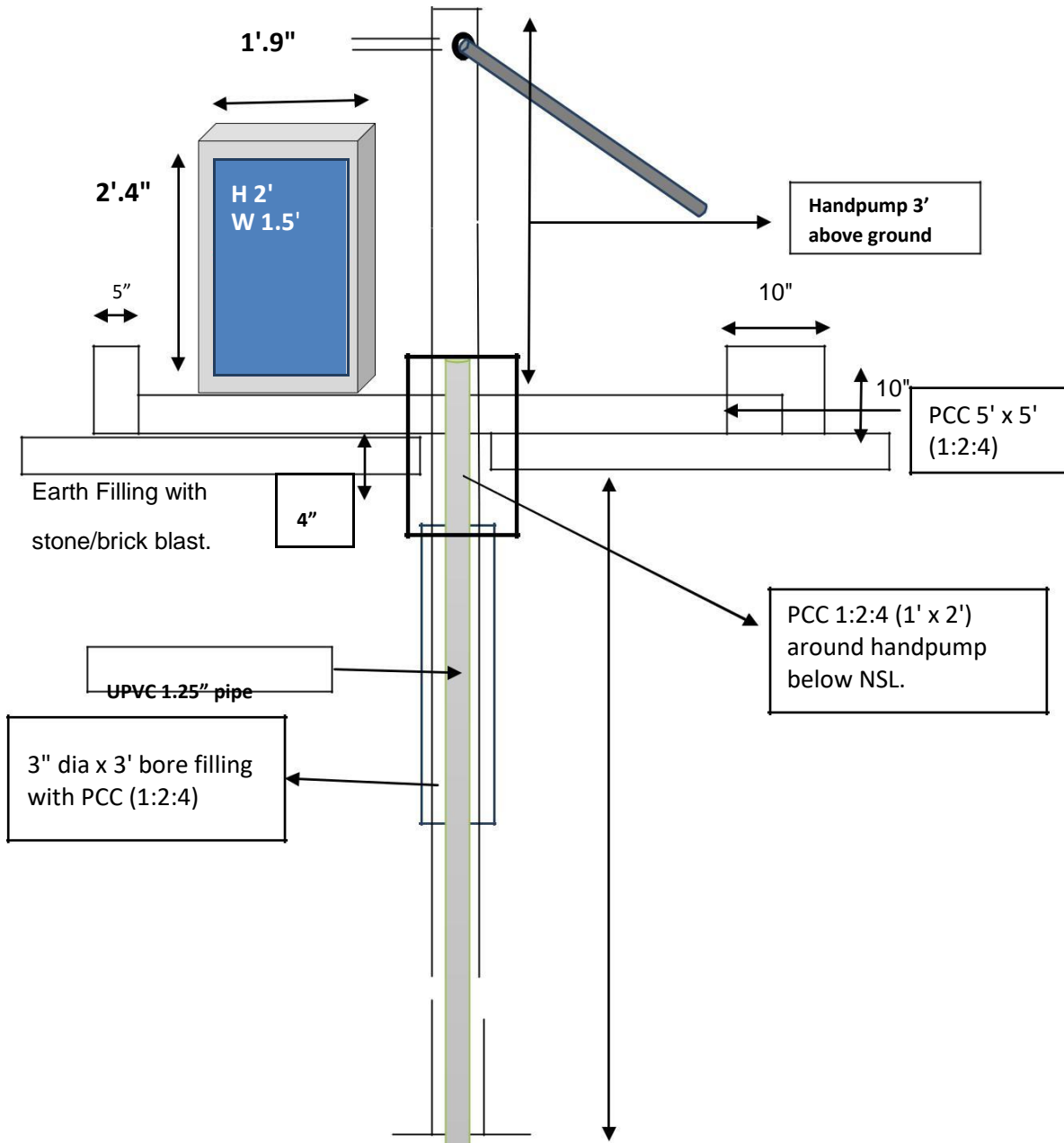
Hand pump Drawing and Plan
